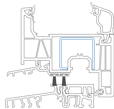
Elegant's warm aluminium threshold with curved slat - Scale 1: 2
