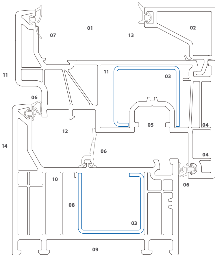
Elegant flush profile Scale 1: 1
