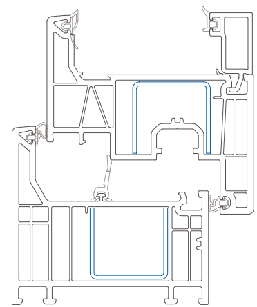
Elegant non-flush profile - Scale 1: 2
